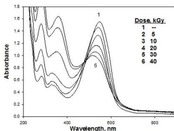
Figure 2. The absorption spectra of CPR/QR/PVA containing chloral hydrate for non-irradiated and irradiated films to different absorbed doses. [CPR] = 0.21 phr, [QR] = 0.42 phr, [Chloral hydrate] = 26.4 phr.
