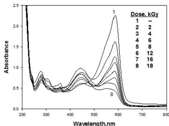
Figure 1. The absorption spectra of CPR/QR/PVA containing chloral hydrate for non-irradiated and irradiated films to different absorbed doses. [CPR] = 0.42 phr, [QR] = 0.21 phr, [Chloral hydrate] = 26.4 phr.
