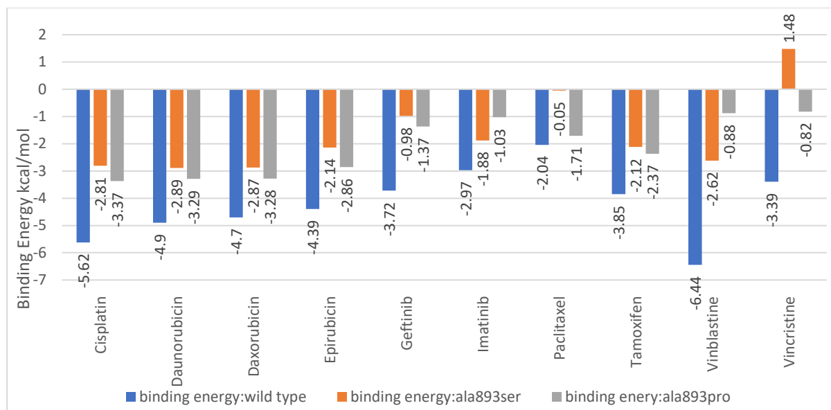
Fig 4: Summary of binding energies of PGP with WILD type, Ala893Ser and Ala893Pro
