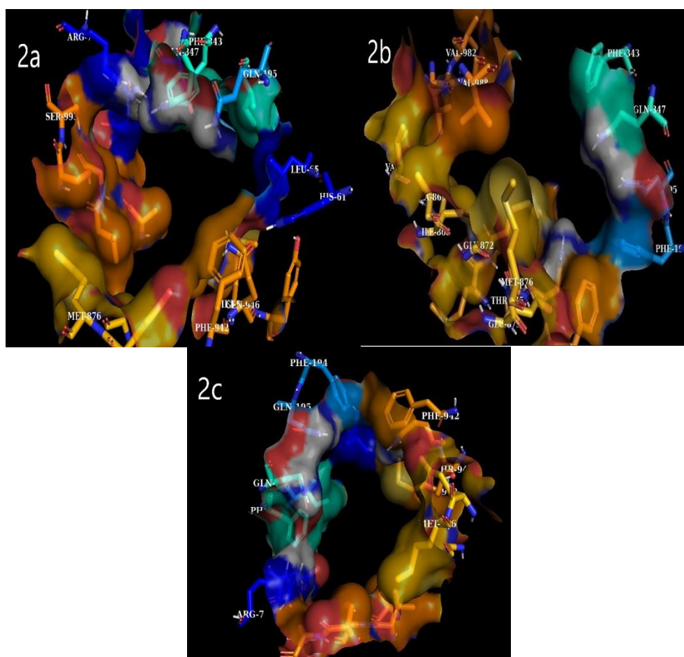
Fig 2: Human PGP Transmembrane Domains involved in Substrate Uptake and Transport
