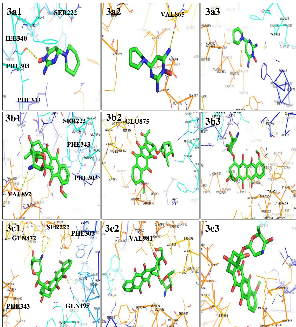
Fig.3: Three dimensional Complexes of Wild and Modeled Mutant PGP structures with docked substrates.
