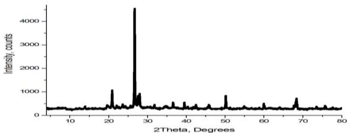
Fig. 4. X-ray diffraction pattern of glauconite sand from the Krantauskoe deposit
