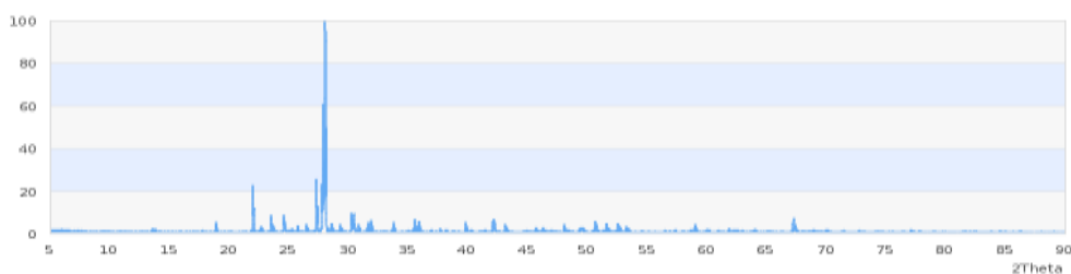
Fig.2. Microcline diffractogram
