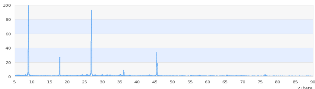
Fig.1. Diffractogram of muscovite
