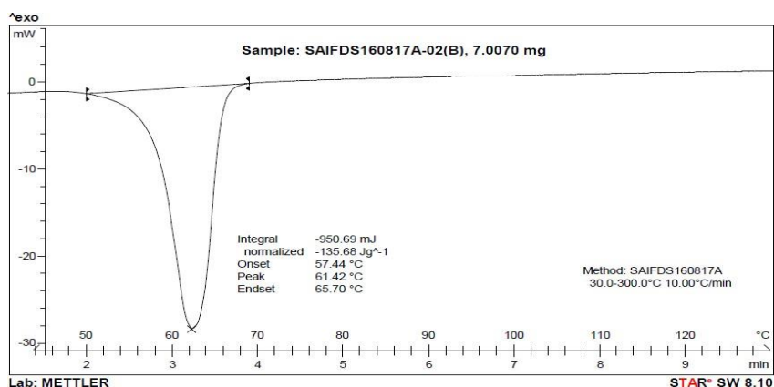
Figure 11: DSC thermogram of Solid dispersions
