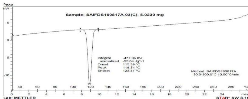
Figure 10: DSC thermogram of Nebivolol
