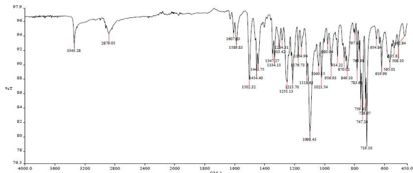
Figure 2: IR spectrum of Nebivolol + PEG 6000
