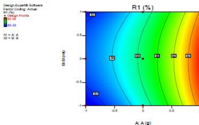
Figure 4: Contour plot for the effect of amount of PEG 6000 and amount of methanol on cumulative percentage release at 60th minute
