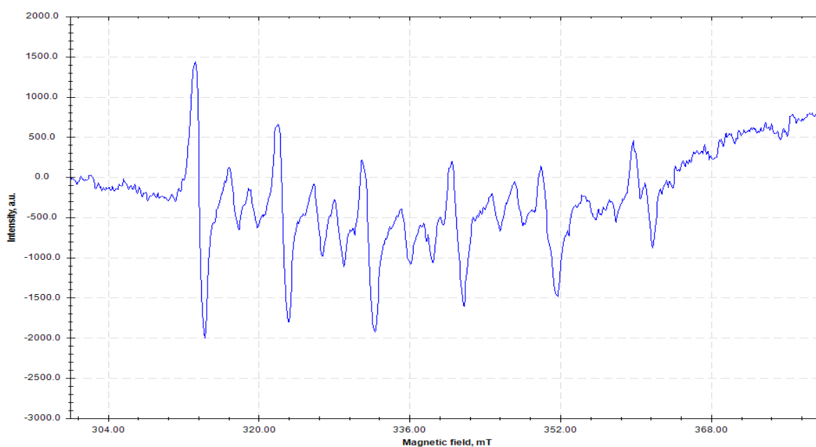
Fig. 1. EPR spectrum [\text{Cr}(\text{AcAc})_2(\text{AA})_2]
