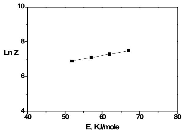
Figure 12. Kinetic compensation effect in Cu(II) complex.
