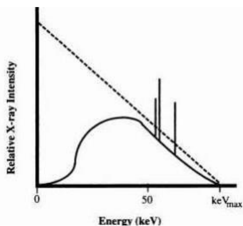
Figure 3. Spectrum of emission to a tungsten target.
