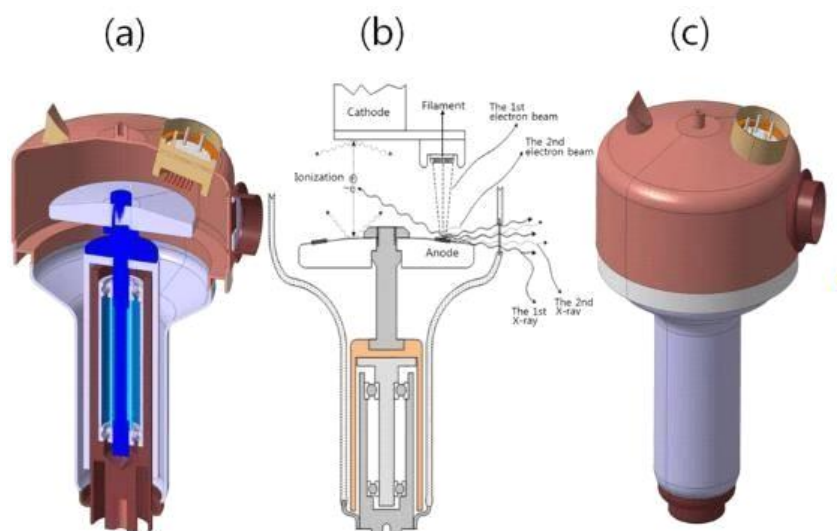
Figure 7. Anode tube
