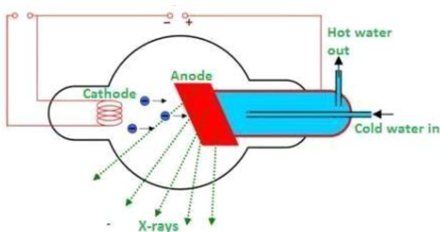
Figure 1. Basic x-ray production process.
