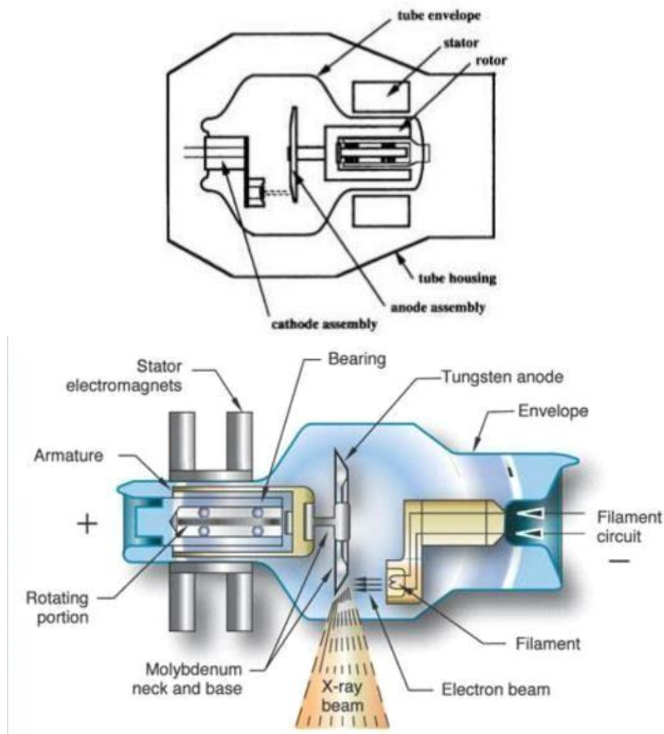
Figure 5. X-ray tube elements
