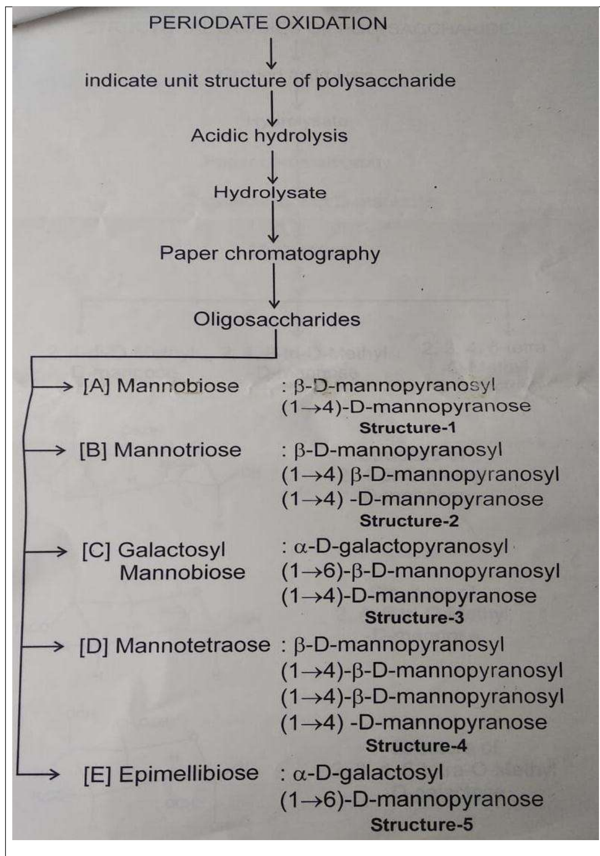
FIG. 5 Structural studies of the purified polysaccharide by peridative oxidation.
