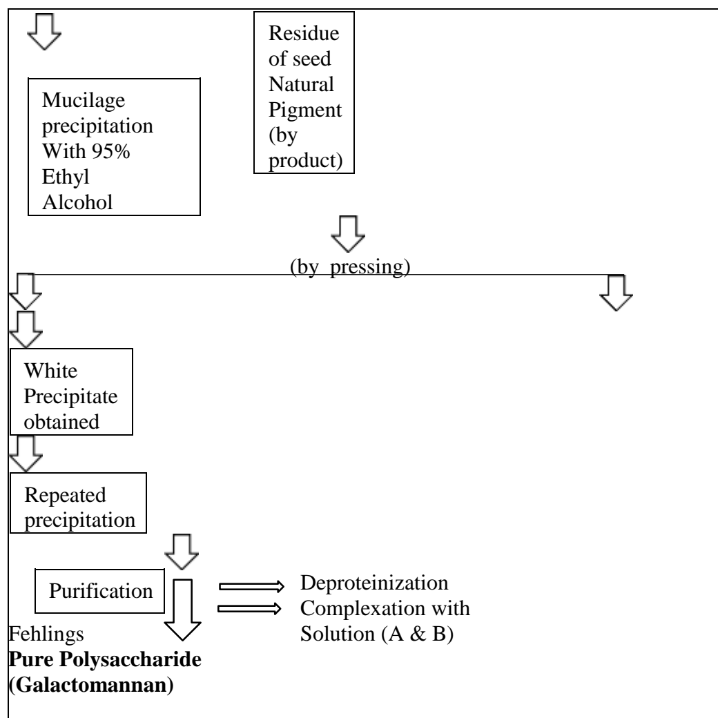
FIG.2 Step by step method for extracting polysaccharide galactomannan from seeds of the plant Leucaena leucocephala and its purification.
