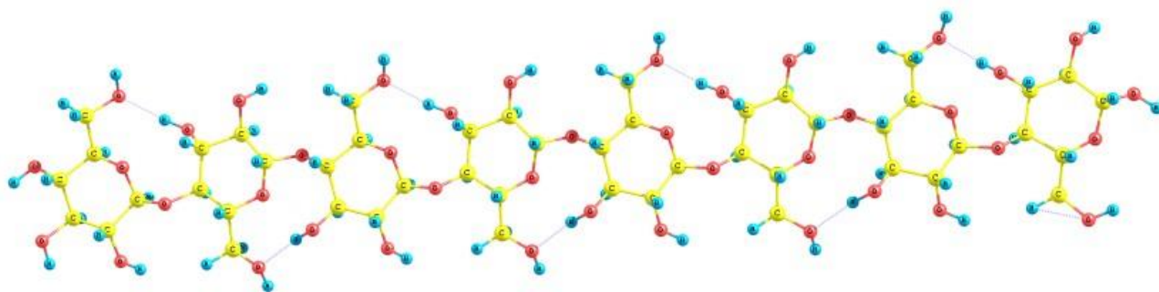
Figure 7. Optimized structure of cellulose (8 glucose units) which is optimized at PM3 semi-empirical quantum mechanical method. COOH is replaced with OH of CH 2 OH.
