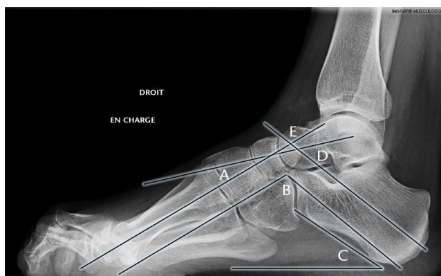
Fig. 1 Radiographic angles on lateral standing radiograph. a) Talo-first metatarsal angle (Meary's angle); b) Djian-Annonier angle less than 120^\circ in cavus foot; c) calcaneal pitch; d) talo-calcaneal angle; e) first metatarsal-calcaneal angle (Hibb's angle).
