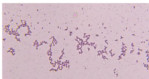
GRAM STAINING
