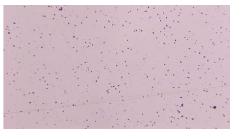
Gram Staining
