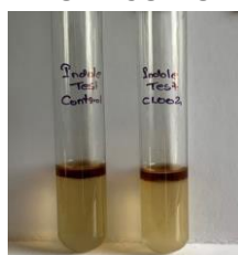
PURE CULTURE
