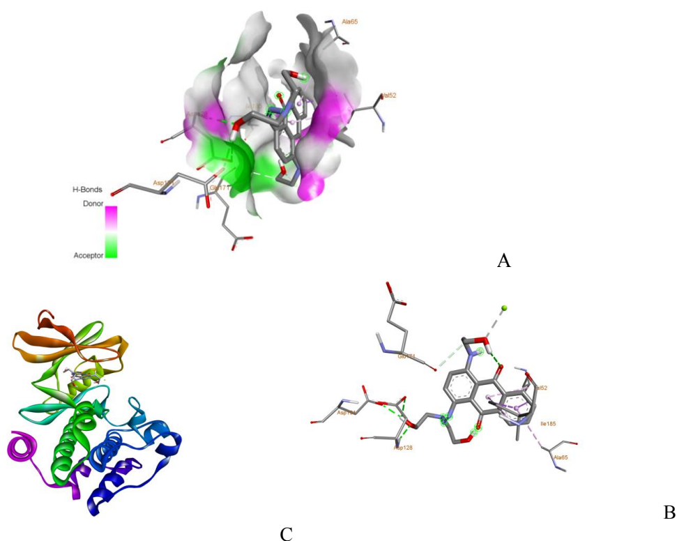
Figure 3: (A) Interaction with the ligand 4 the H-bond surfaces of the receptor COVID-19 inhibitor (B) The docked ligand triazene 4 at the same catalytic site receptor, (C) 3D Docking poses of compound 3 into the N3 binding site of the COVID-19 main protease
