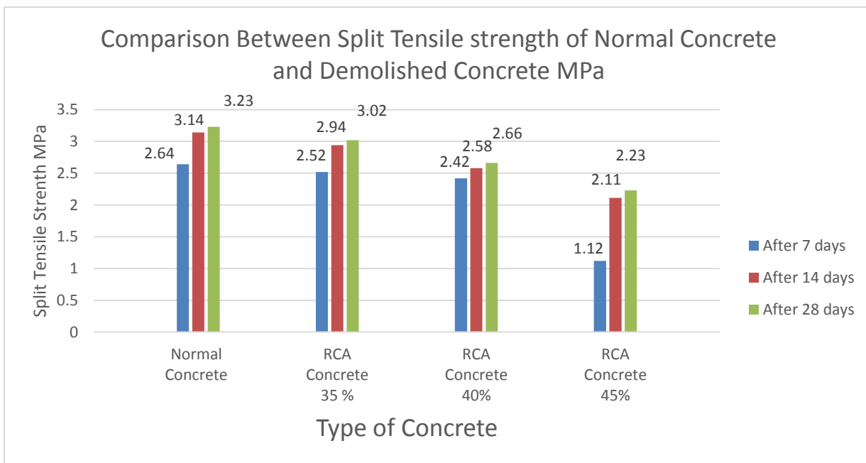
Fig. 6 Exploratory Split tensile strength Test Comparison Chart
