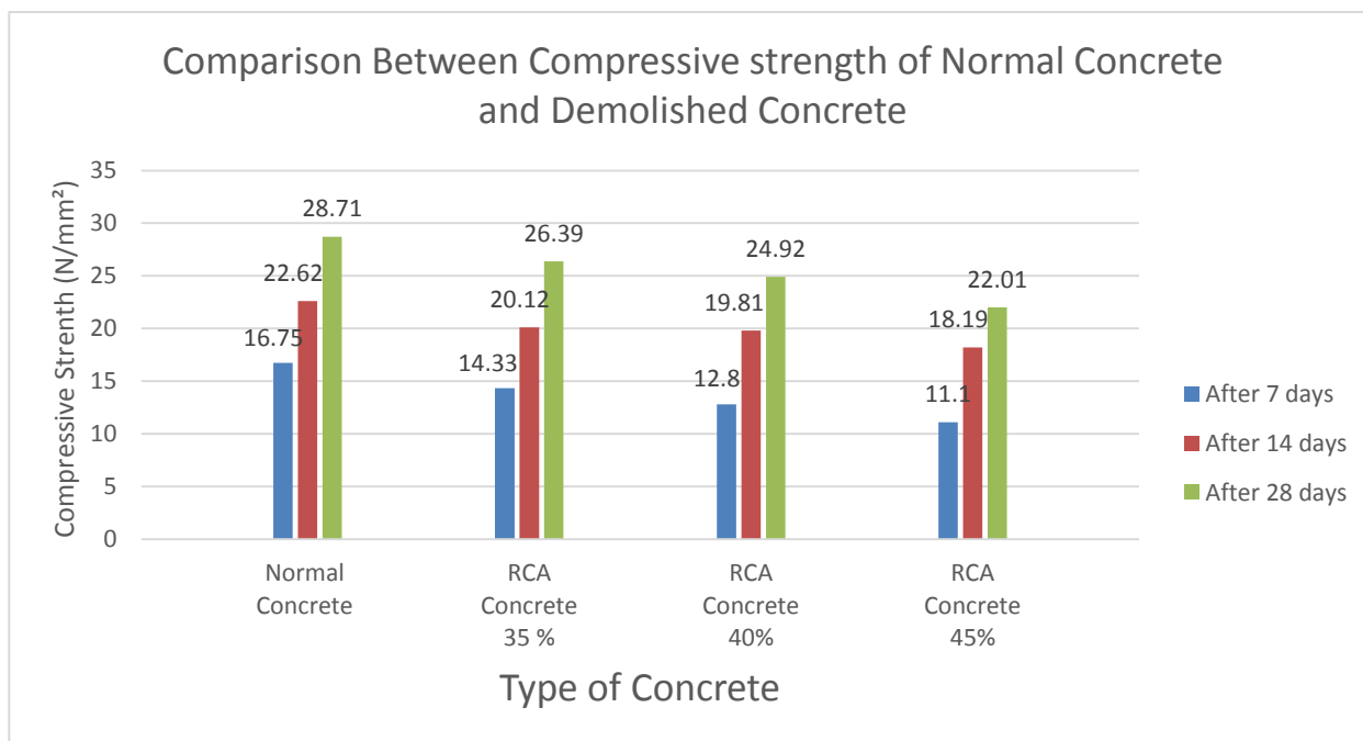
Fig. 5 Exploratory Compressive strength Test Comparison Chart
