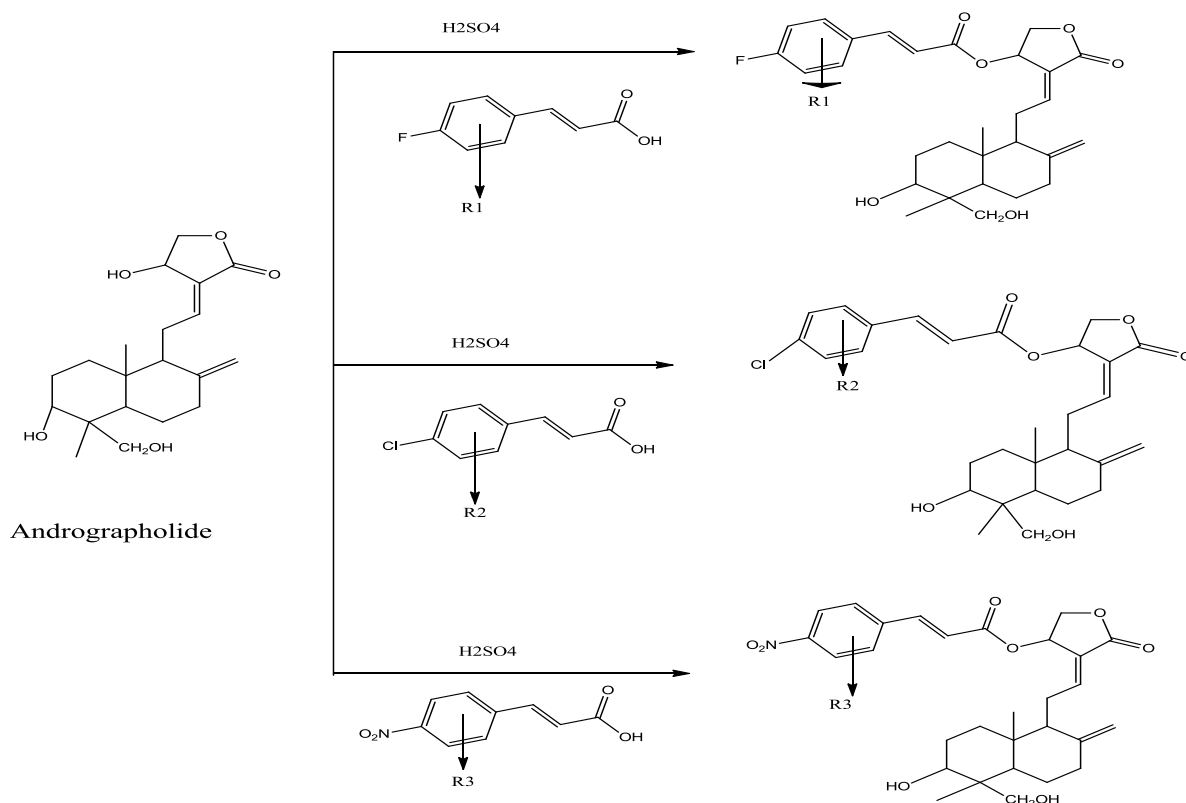
Andrographolide analogous
