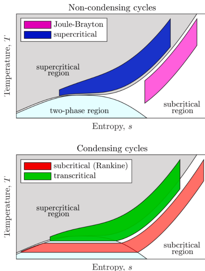
Figure 1 Classification of thermodynamic power cycles[17]
