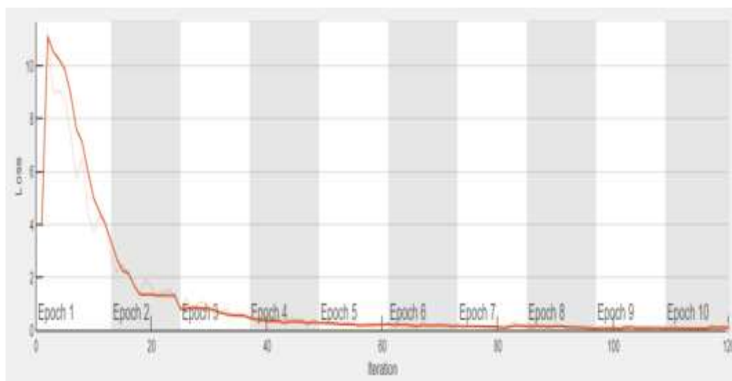
Fig 3 Loss computation
