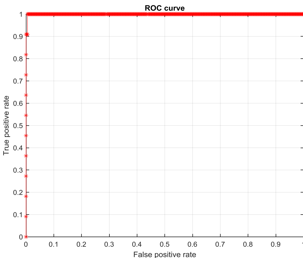
Fig 6 ROC curve
