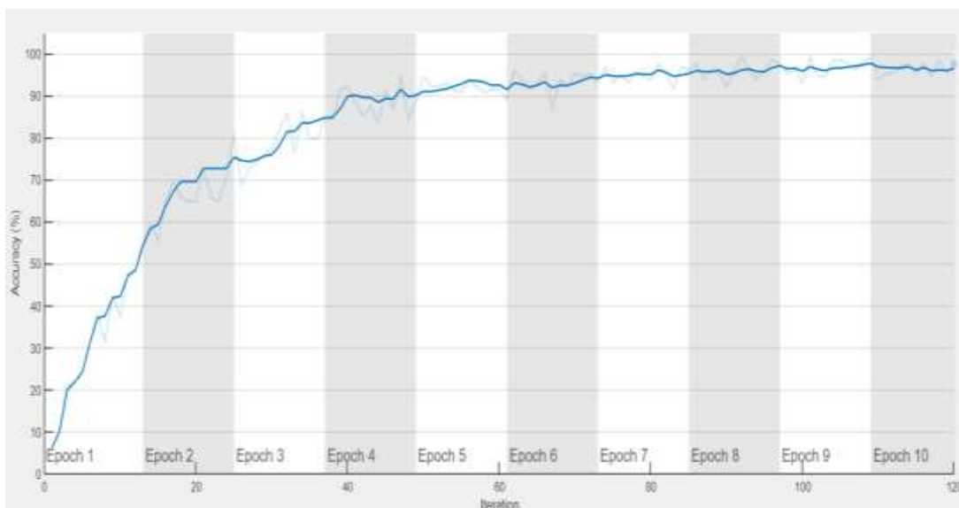
Fig 2 Accuracy computation
