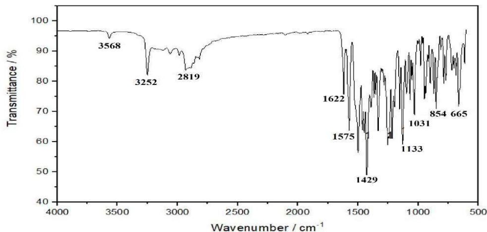
Figure 3: FTIR spectra of pure drug Erlotinib
