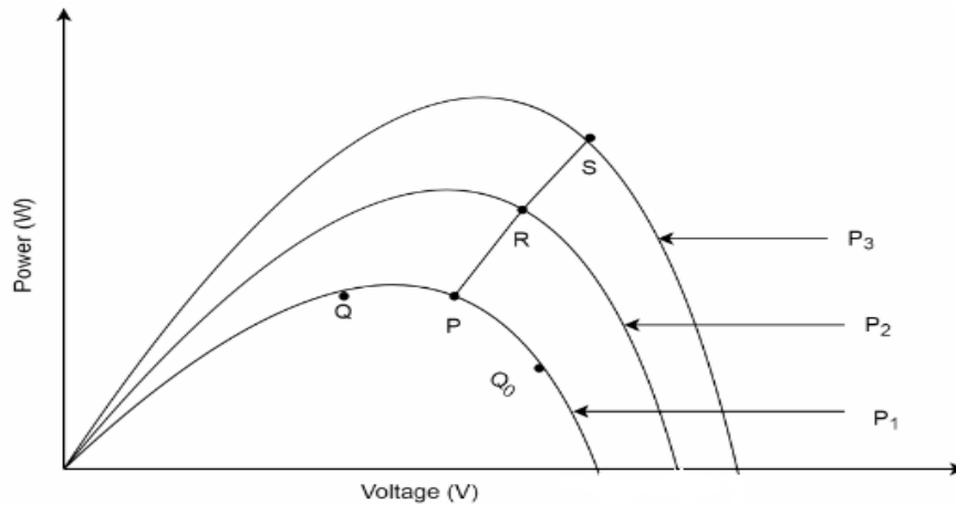
Fig.5 Operation of P & O MPPT Technique
