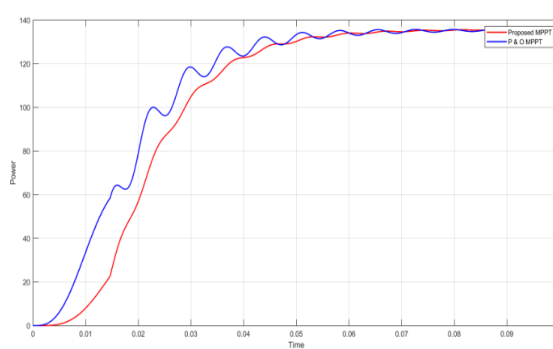
Fig. 10 Pattern 4 curve for 2S3P Configuration
