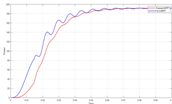
Fig. 9 Pattern 3 curve for 2S3P Configuration
