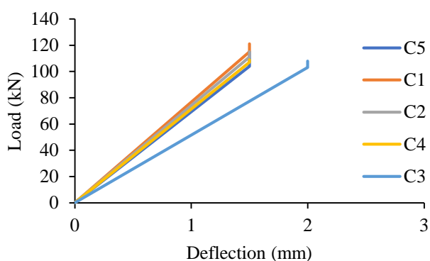
Fig. 12 Graph of Load vs deflection for model I from table 8.
