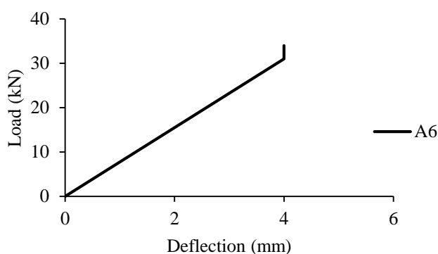
Fig. 7 Graph of Load vs deflection for model III from table 6.
