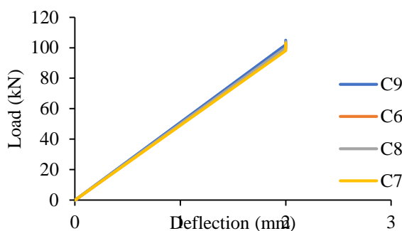
Fig. 11 Graph of Load vs deflection for model II from table 8.
