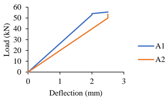
Fig. 5 Graph of Load vs deflection for model I from table 6.
