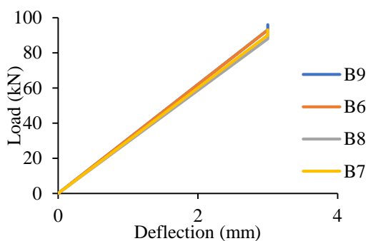
Fig. 8 Graph of Load vs deflection for model II from table 7.
