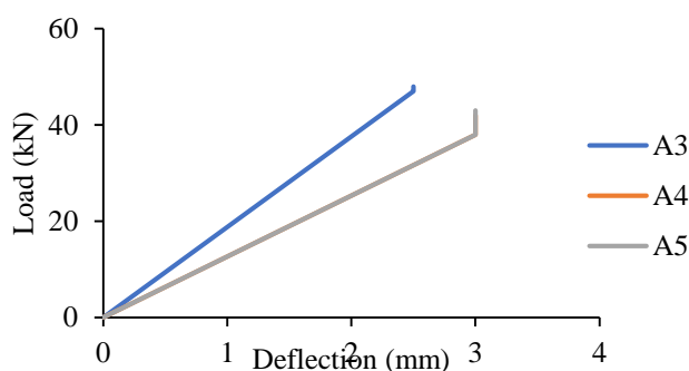
Fig. 6 Graph of Load vs deflection for model II from table 6.
