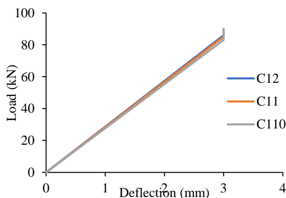
Fig. 13 Graph of Load vs deflection for model III from table 8.
