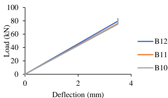
Fig. 10 Graph of Load vs deflection for model III from table 7.
