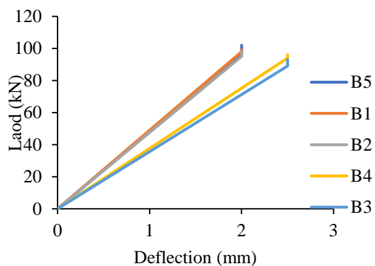
Fig. 9 Graph of Load vs deflection for model I from table 7.
