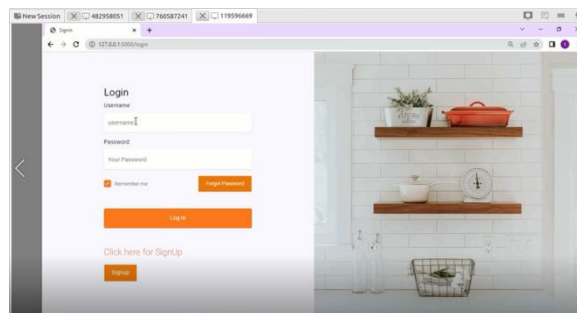
Fig.5: User signin
