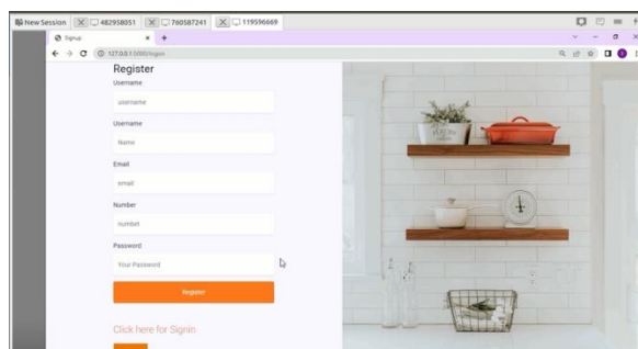
Fig.4: User signup
