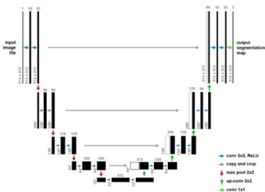
Fig.2: System architecture
