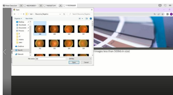
Fig.7: User input
