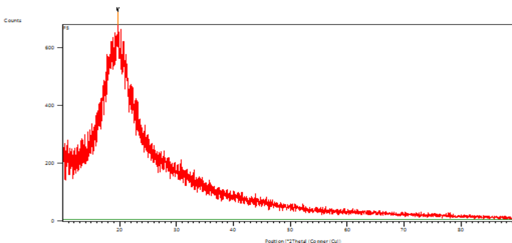
FIG.4 XRD spectra
