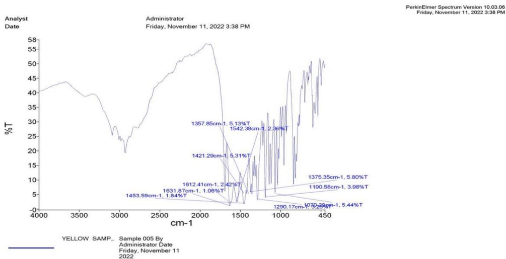
Fig.2: FTIR spectra of usnic acid
