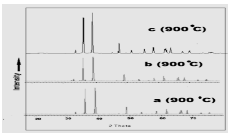
Fig 1: XRD patterns of as-prepared CuO NPs samples using different solvents (a) water (b) water-methanol (c) water-ACN
