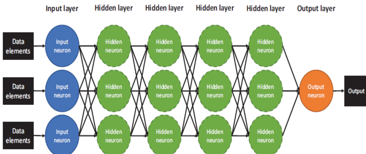
Fig 8: Example of a deep neural network, a subtype of neural networks with multiple hidden layers between the input and output layers. The outputs from one layer of neurons becomes the inputs for the next layer of neurons.
