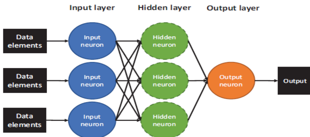
Fig 7: Example of a neural network. A neural network connects several “neurons” (linear models) together, where the outputs form one layer become the inputs for the next. The input layer processes the raw data inputs and then passes the results to the next layer (hidden layer) for additional processing, with the results then passed to the output neuron to obtain the final result.
