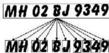
Fig4.1.3 Character Segmentation
