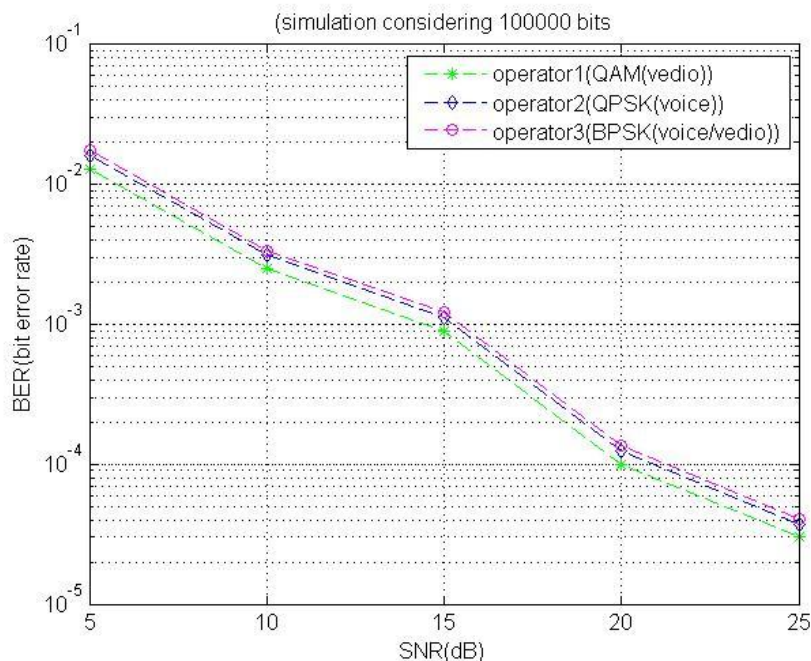
Fig 4.6: BER (bit error rate) and SNR (dB)
