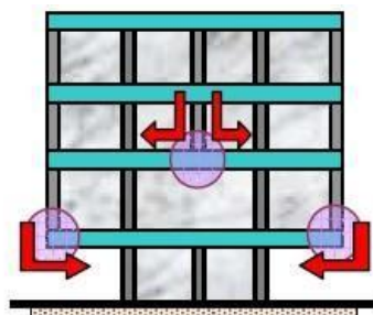
Hanging or Floating Columns
