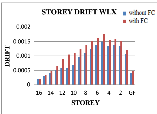
STOREY DRIFT WLX
