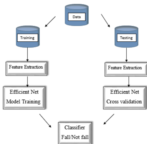
Fig 3: Fall detection process
