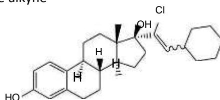
Figure 2. 17 \alpha -(19-chlorovinilic-20 cyclohexane)estradiol.
