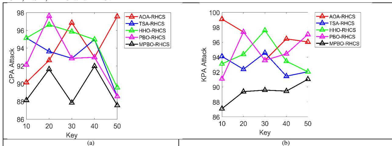
Fig.4. (a) CPA attack
