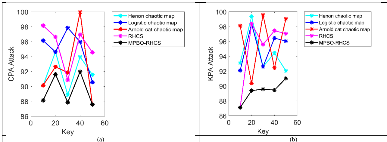
Fig.8. (a) CPA attack (b) KPA attack
