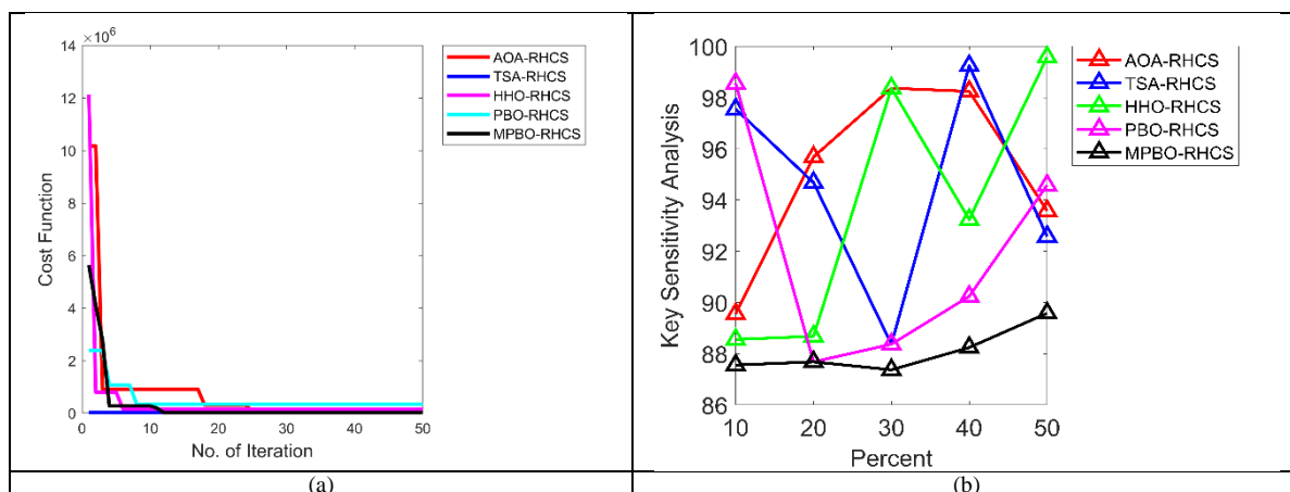
Fig.5. (a) convergence analysis
