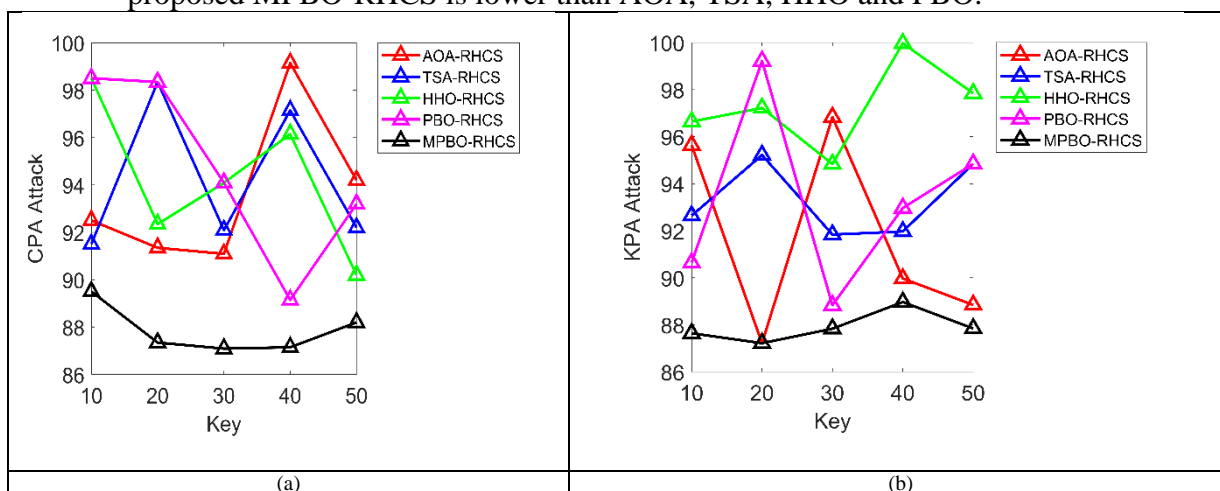
Fig.6. (a) CPA attack
